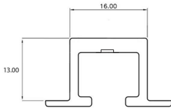
FLUSH FIT TRACK PROFILE
